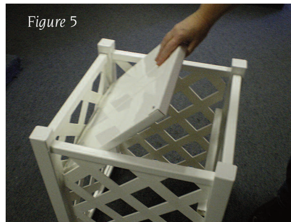
Figure #5. After all sides are assembled set shelf on top of rails.
