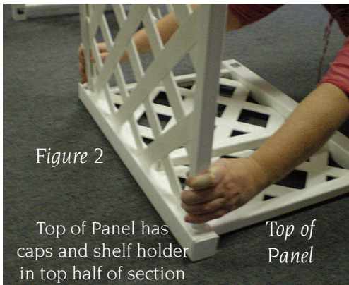
Figure #2. Take your first (A) Solid side panel, (be sure to have shelf bar towards top) Place in routed holes, shoving channels on lattice insert all the way down, to form a snug fit with other channel inside post. See figure #3
